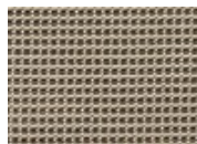
858 Theoretical Model
