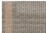
847 Reshape
